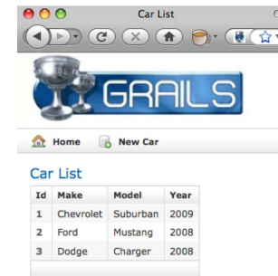
Figure 2: Car List
