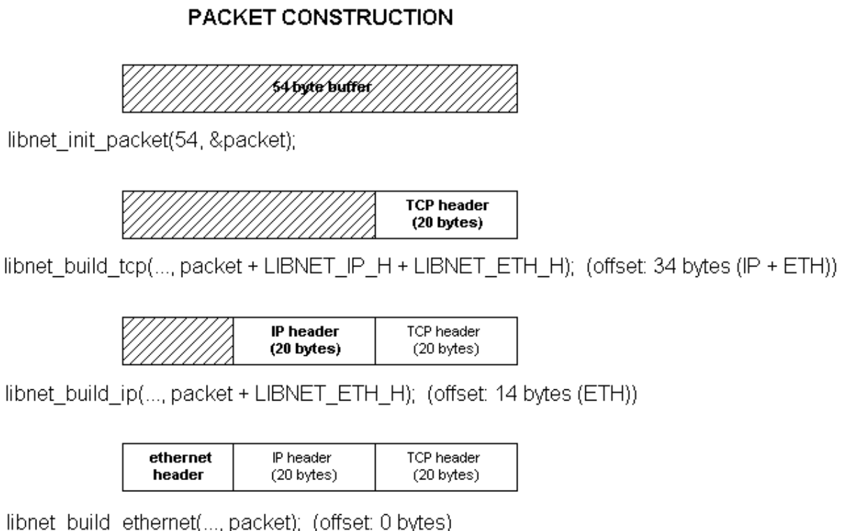
Figure 4. Modular Packet Construction
