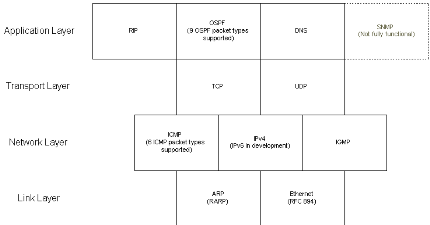
Figure 1. Libnet Supported Protocols
