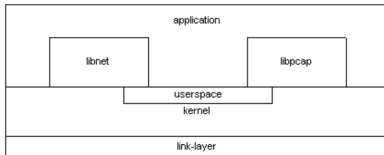
Figure 2. Application layering with libnet and libpcap
