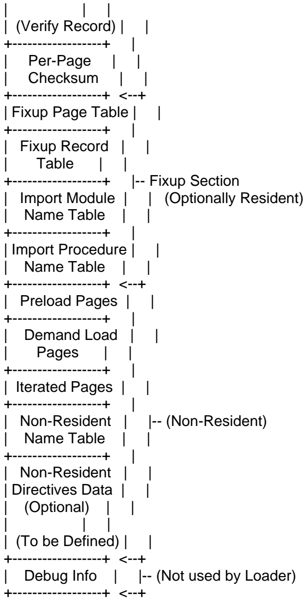
Figure 2. 32-bit Linear EXE Header
