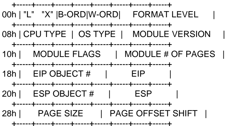
Figure 2. 32-bit Linear EXE Header
