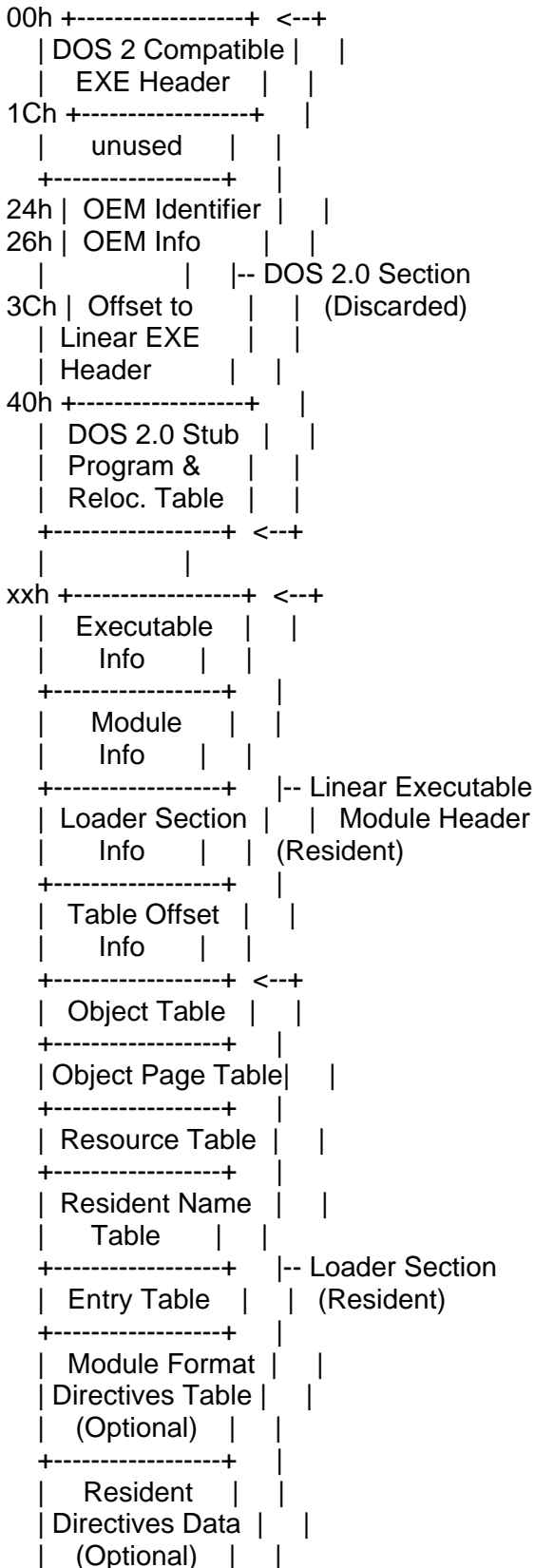
Figure 1. 32-bit Linear EXE File Layout
