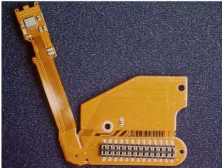
Figure 9 – Disk Drive Flex with Flip Chip
