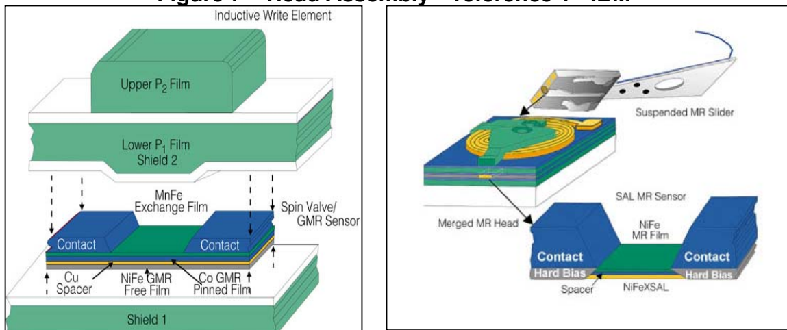
Figure 7 – Head Assembly – reference 1 - IBM
