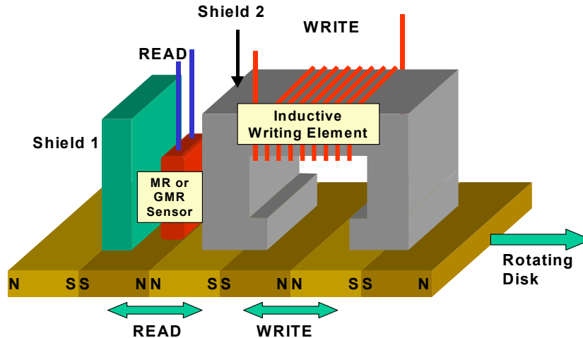
MERGED READ-WRITE HEAD Figure 4
