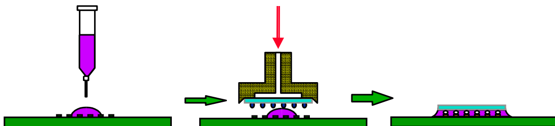
Figure 10 – Pre-Applied Flux/Underfill Process
