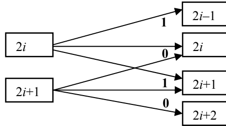
Figure 1b. \pm 1 embedding operation
