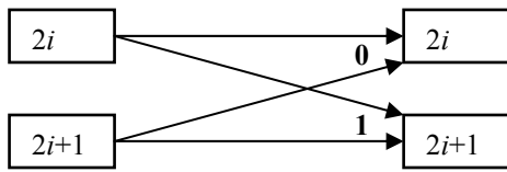
Figure 1a. LSB embedding operation
