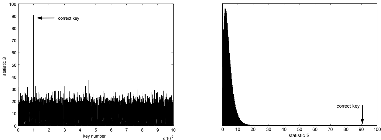
Figure 2. Statistic S (3) (left) and its PDF (right) generated from 2^{20} keys K_j
