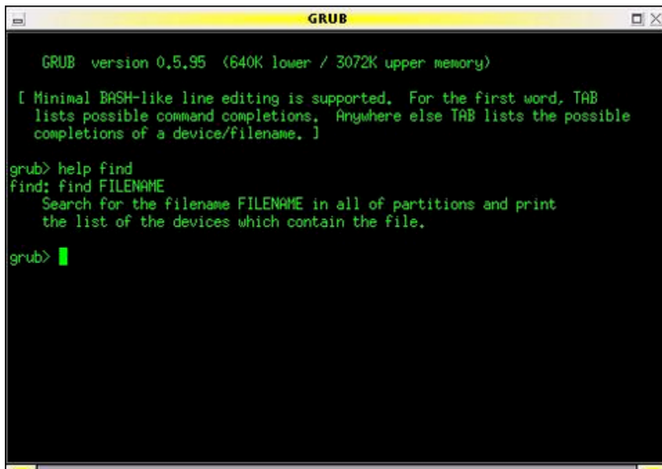
Figure 1. GRUB in command-line mode. Note the on-line help (here the GRUB emulator is running under Linux in an xterm window).
