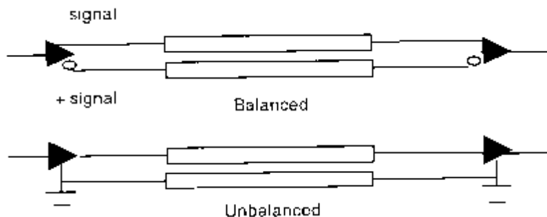
Figure 1: Balanced vs. unbalanced transmission
