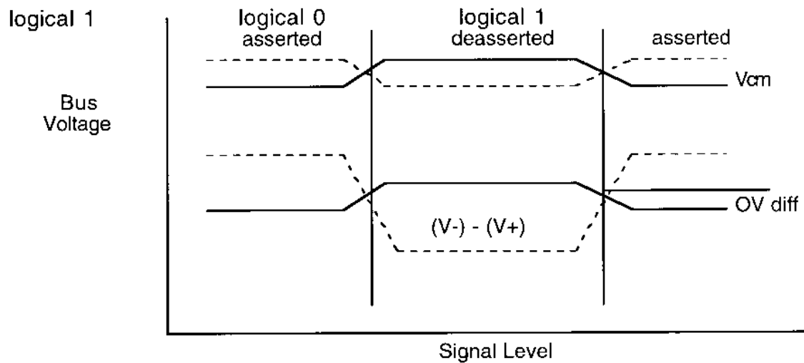
Fig. 3: LVD Signal polarities
