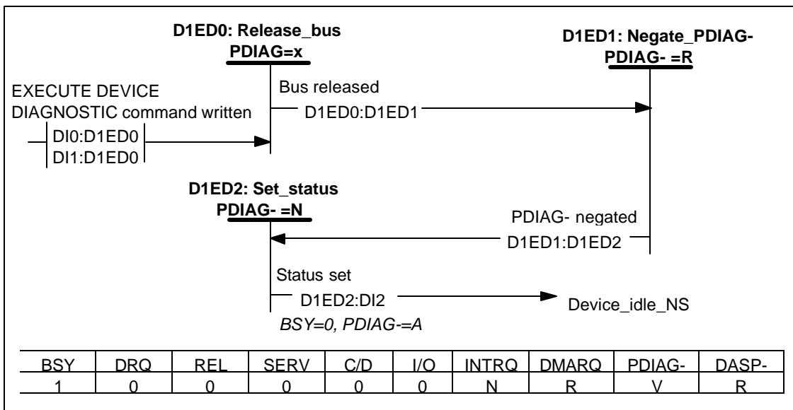
Figure 38 - Device 1 EXECUTE DEVICE DIAGNOSTIC command state diagram
