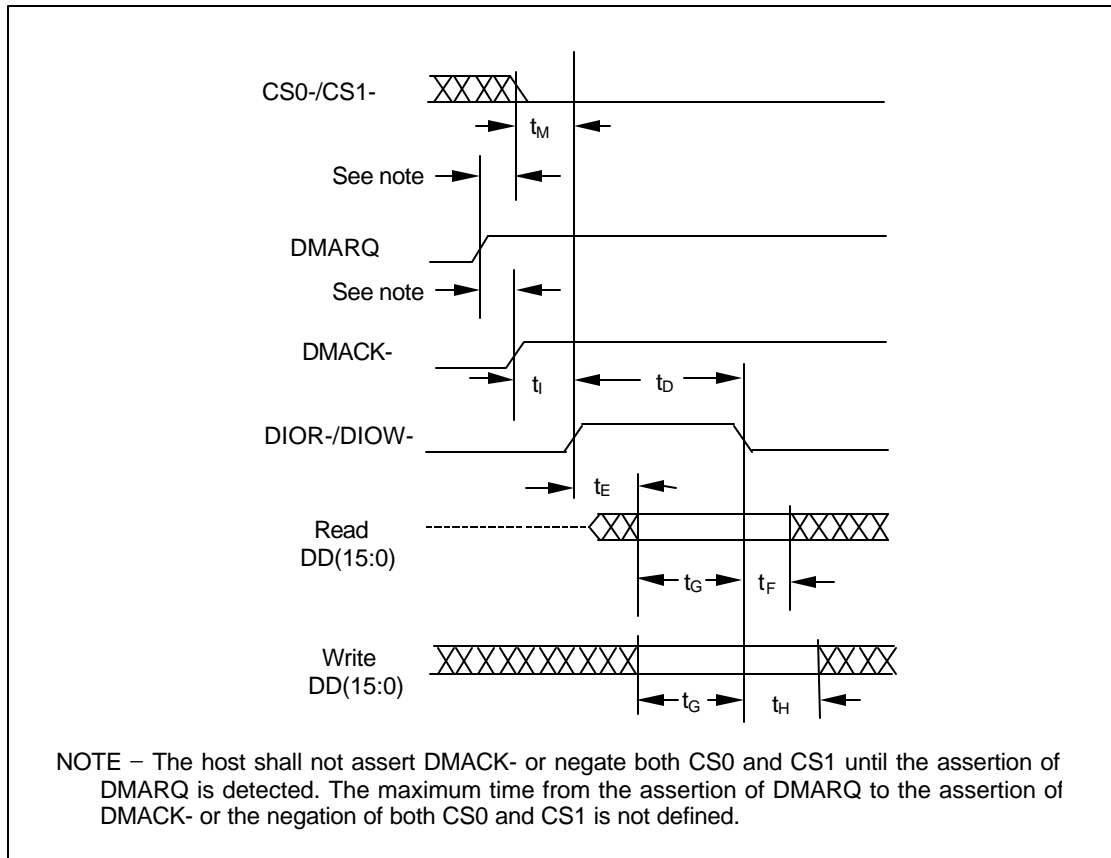
Figure 44 - Initiating a Multiword DMA data transfer
