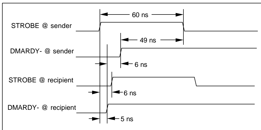
Figure C.31 – STROBE and DMARDY- at sender and recipient
