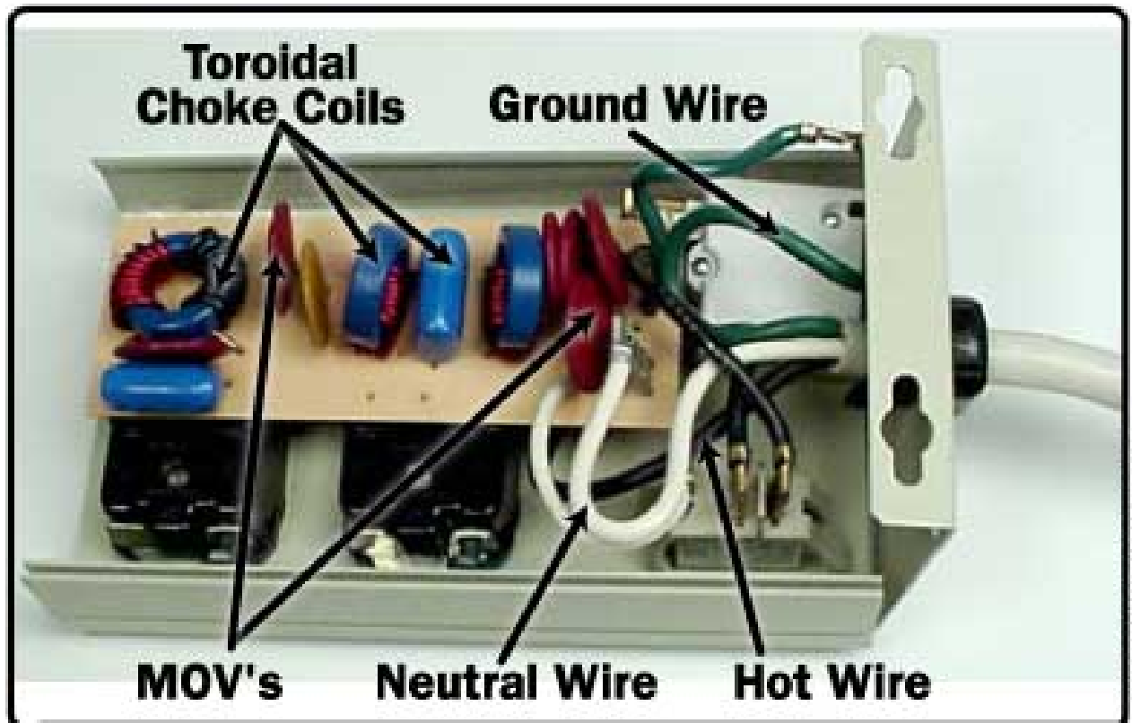
Inside a surge protector with line-conditioning chokes
