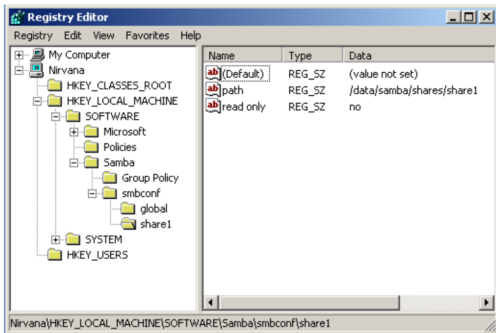
Figure 1: Editing samba configuration with regedit.exe
