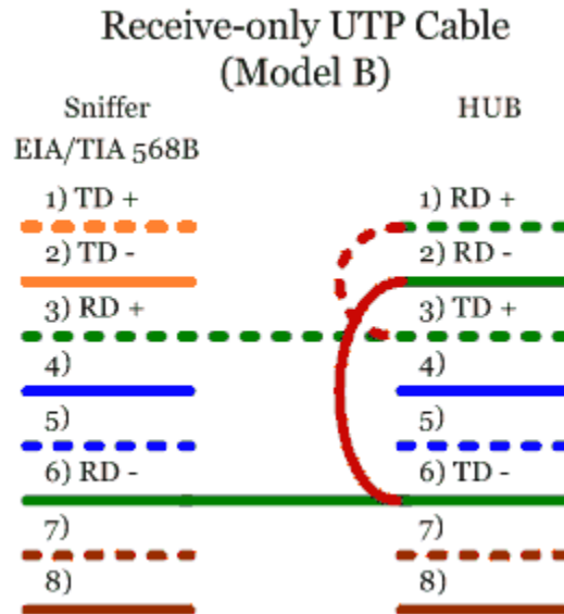
Figure 7: Model B Wiring Scheme
