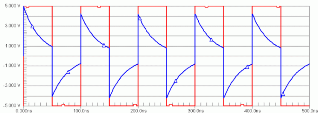
Figure 6: Model A Signal Simulation
