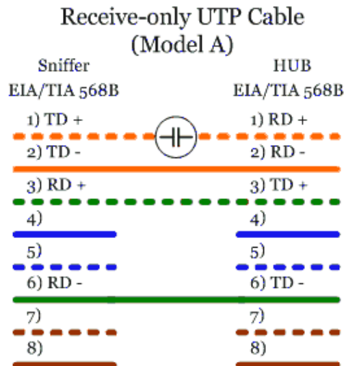
Figure 5: Model A Wiring Scheme
