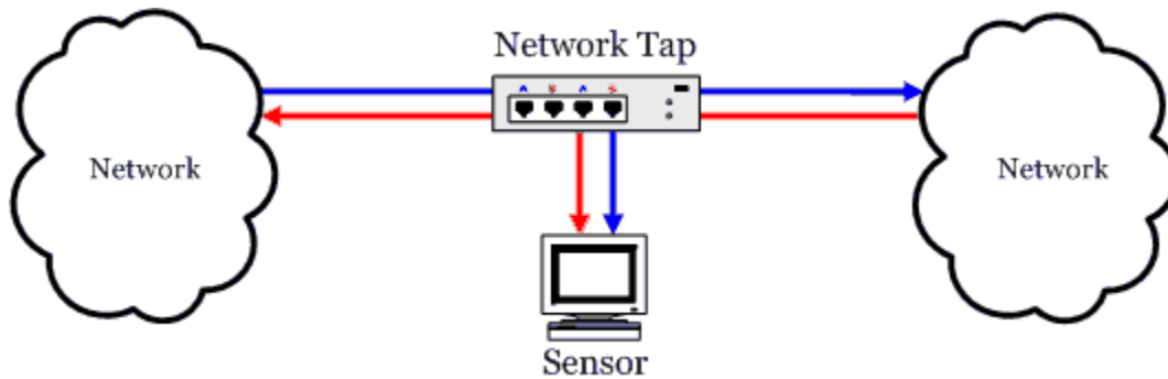
Figure 15: Passive Network Monitoring
