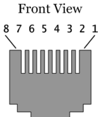
Figure 1: Front view of a RJ45 connector
