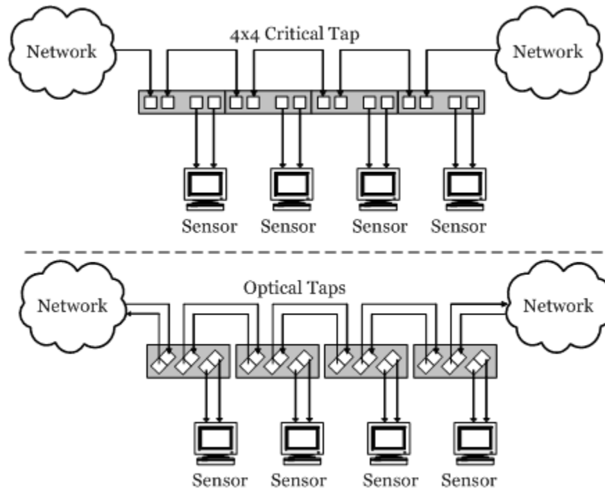
Figure 14: Regeneration Tap using individual Taps
