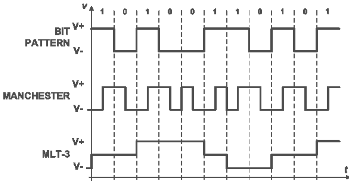
Figure 4: Ethernet Encoding Schemes
