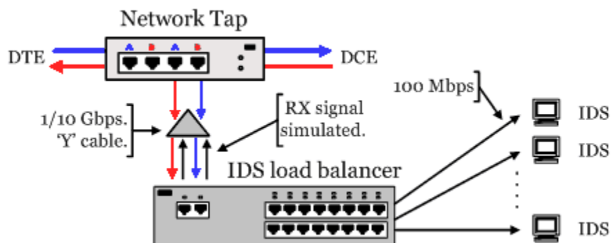
Figure 17: High speed traffic analysis
