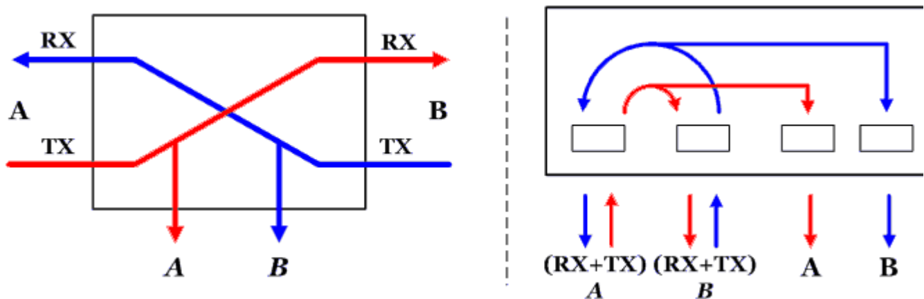
Figure 11: TAP Connection Scheme
