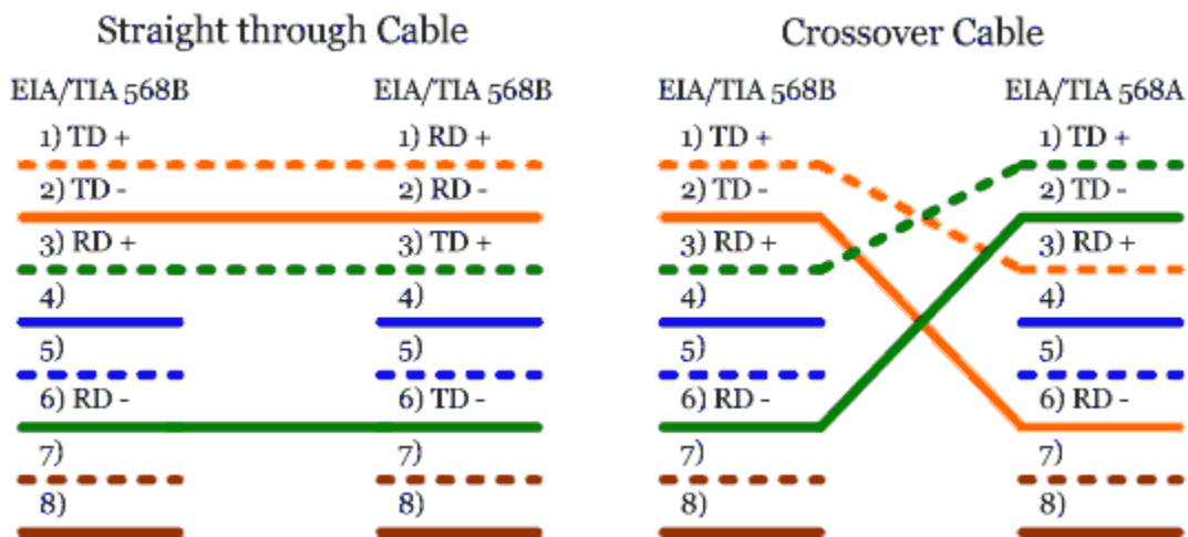
Figure 3: Straight through and crossover wiring schemes (10/100Base-T)
