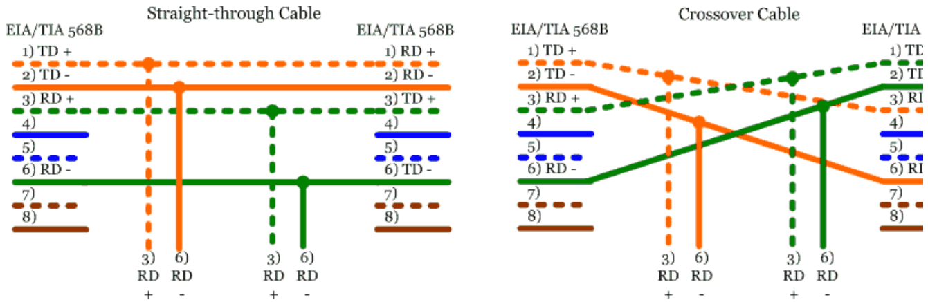
Figure 12: Ethernet TAP Connection Diagrams
