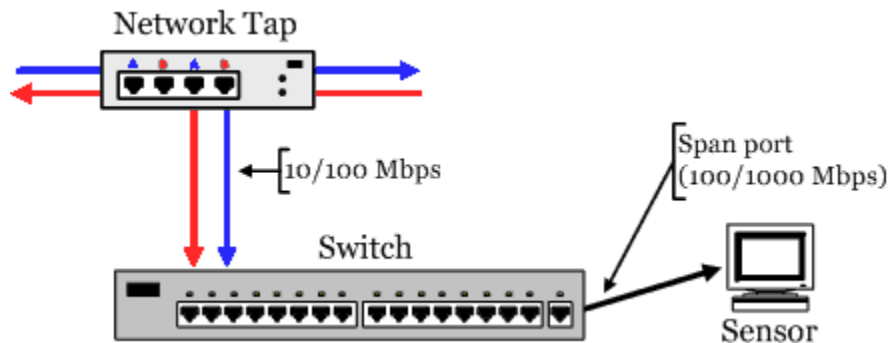
Figure 16: Network Tap and Switch with Span Port
