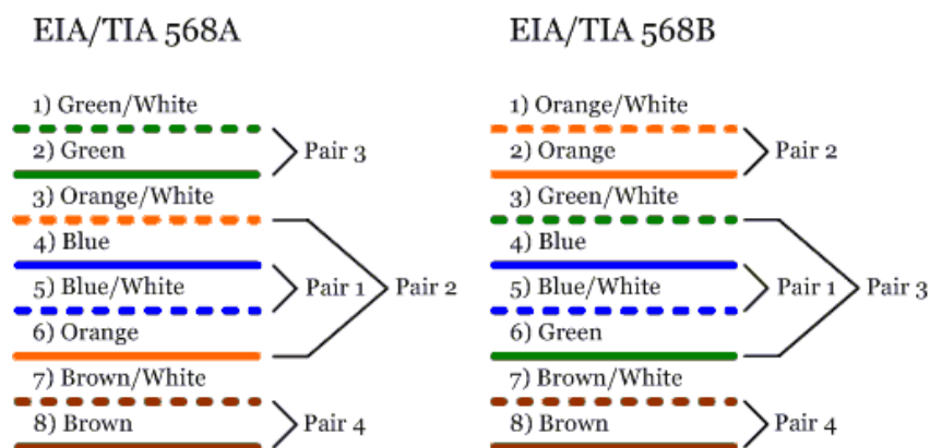
Figure 2: EIA/TIA 568A and 568B norms
