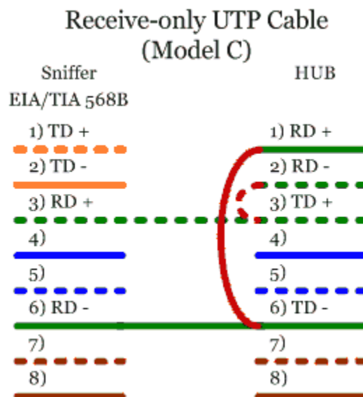
Figure 8: Model C Wiring Scheme
