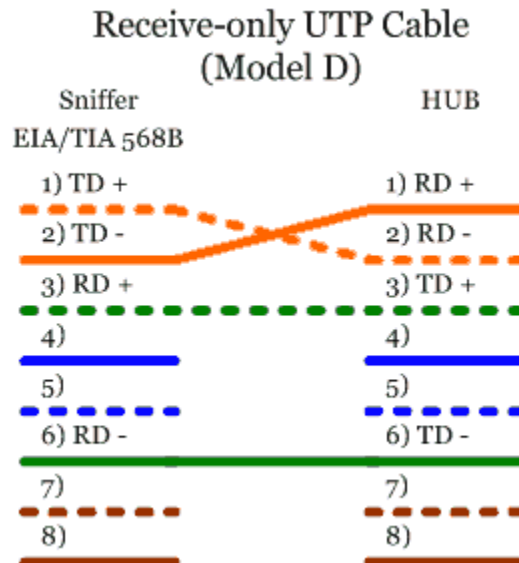
Figure 9: Model D Wiring Scheme
