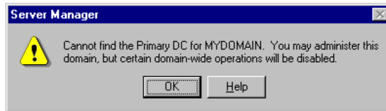
Figure 16: Error Message
